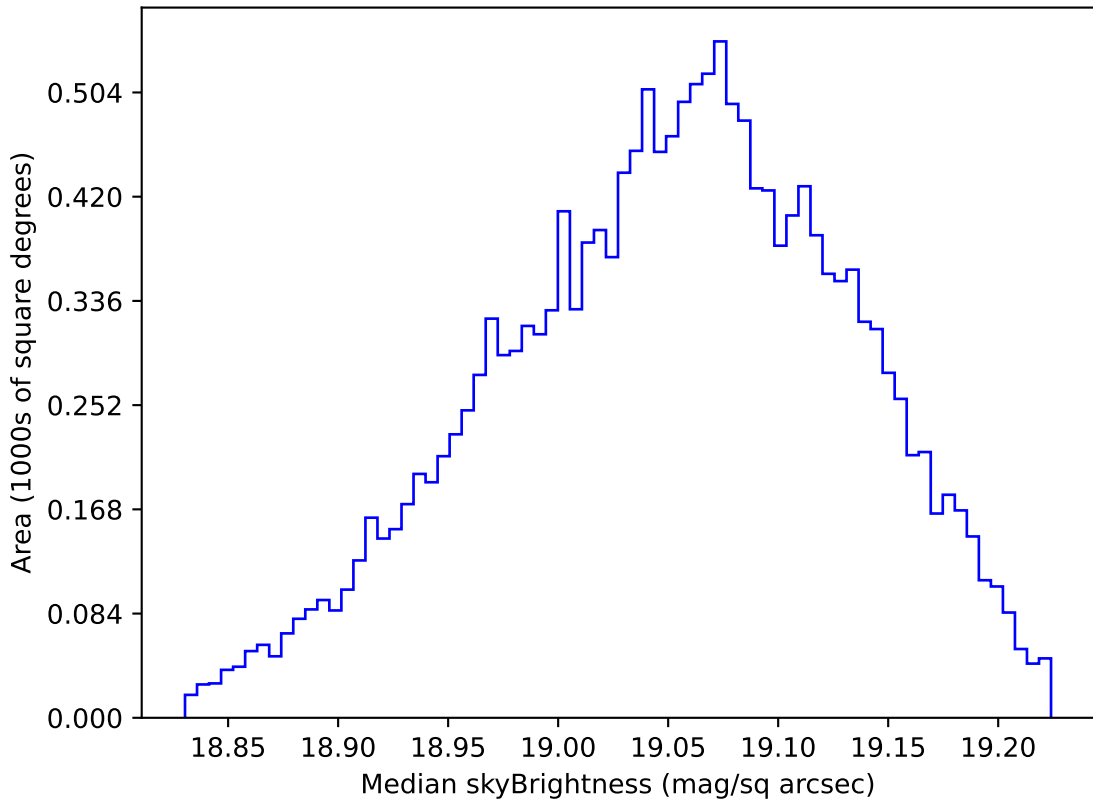
too_elab_r64_d3_gz_v3.4_10yrs WFD z band: Median skyBrightness
