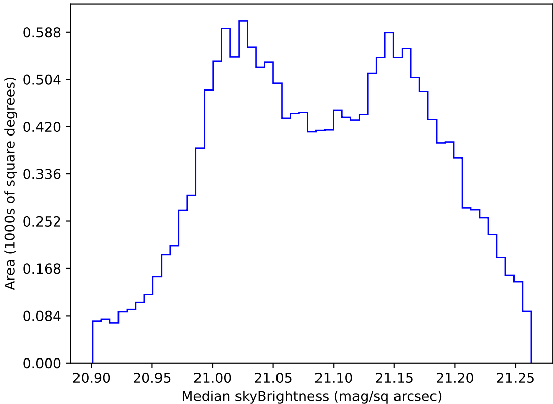
too_elab_r64_d3_gz_v3.4_10yrs WFD r band: Median skyBrightness
