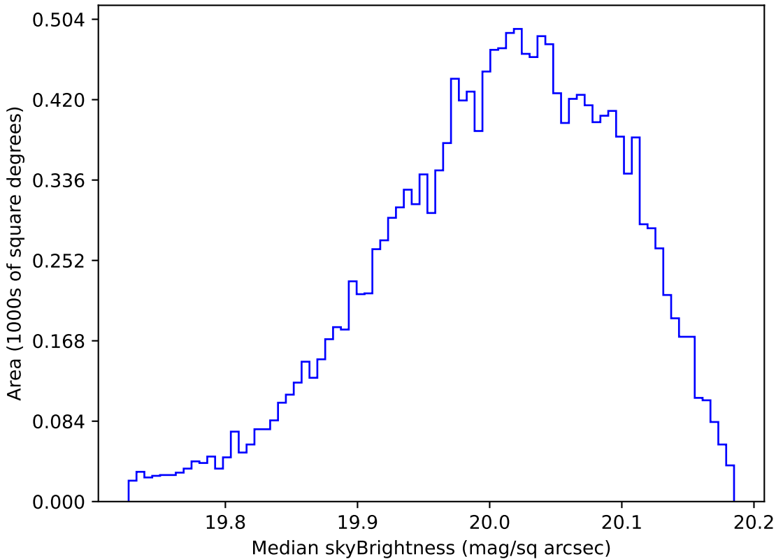
too_elab_r64_d3_gz_v3.4_10yrs WFD i band: Median skyBrightness
