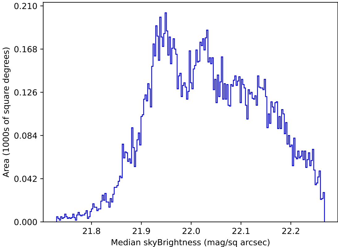
too_elab_r64_d3_gz_v3.4_10yrs WFD g band: Median skyBrightness
