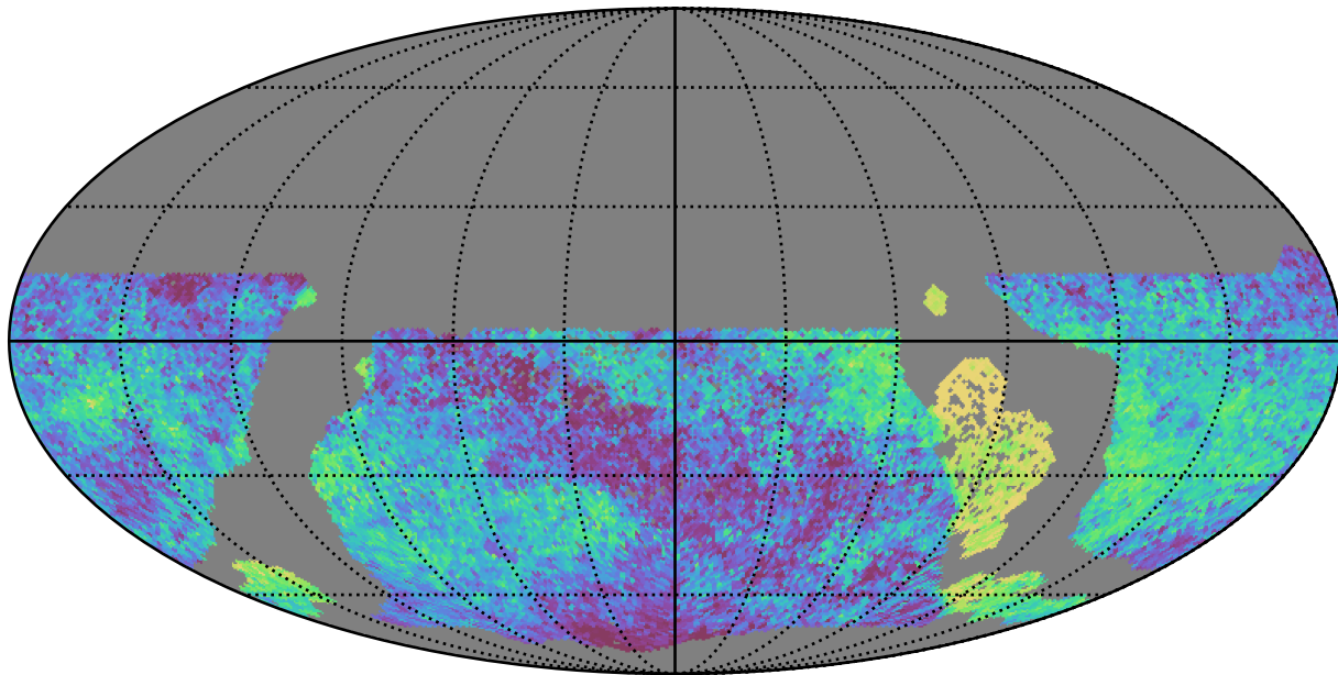
too_elab_r64_d3_gz_v3.4_10yrs WFD all bands: Median skyBrightness
