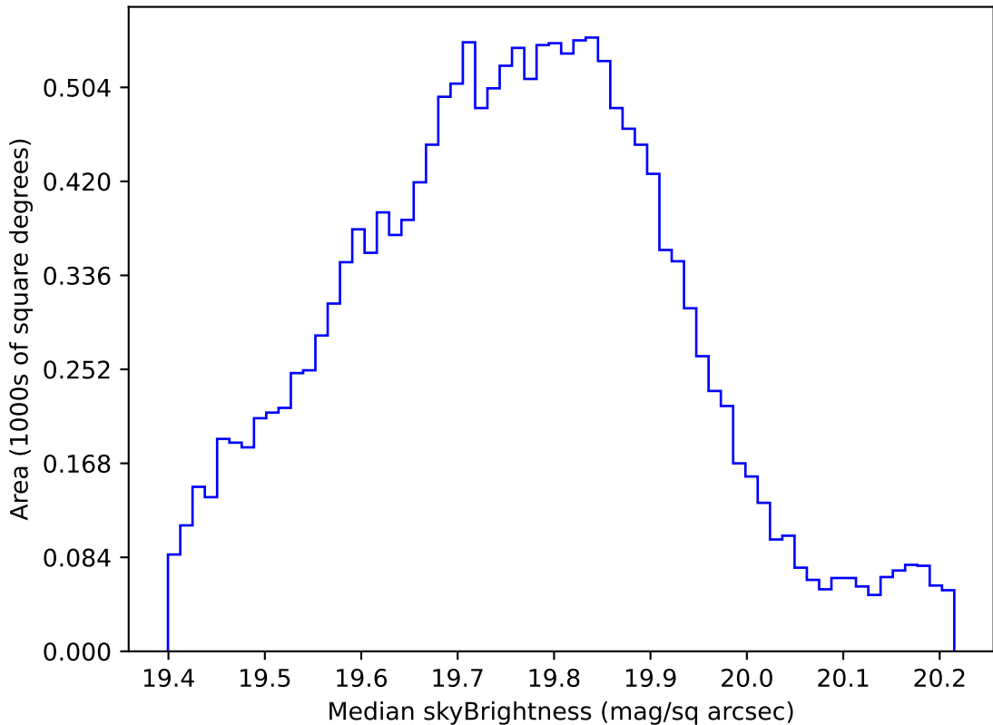
too_elab_r64_d3_gz_v3.4_10yrs WFD all bands: Median skyBrightness
