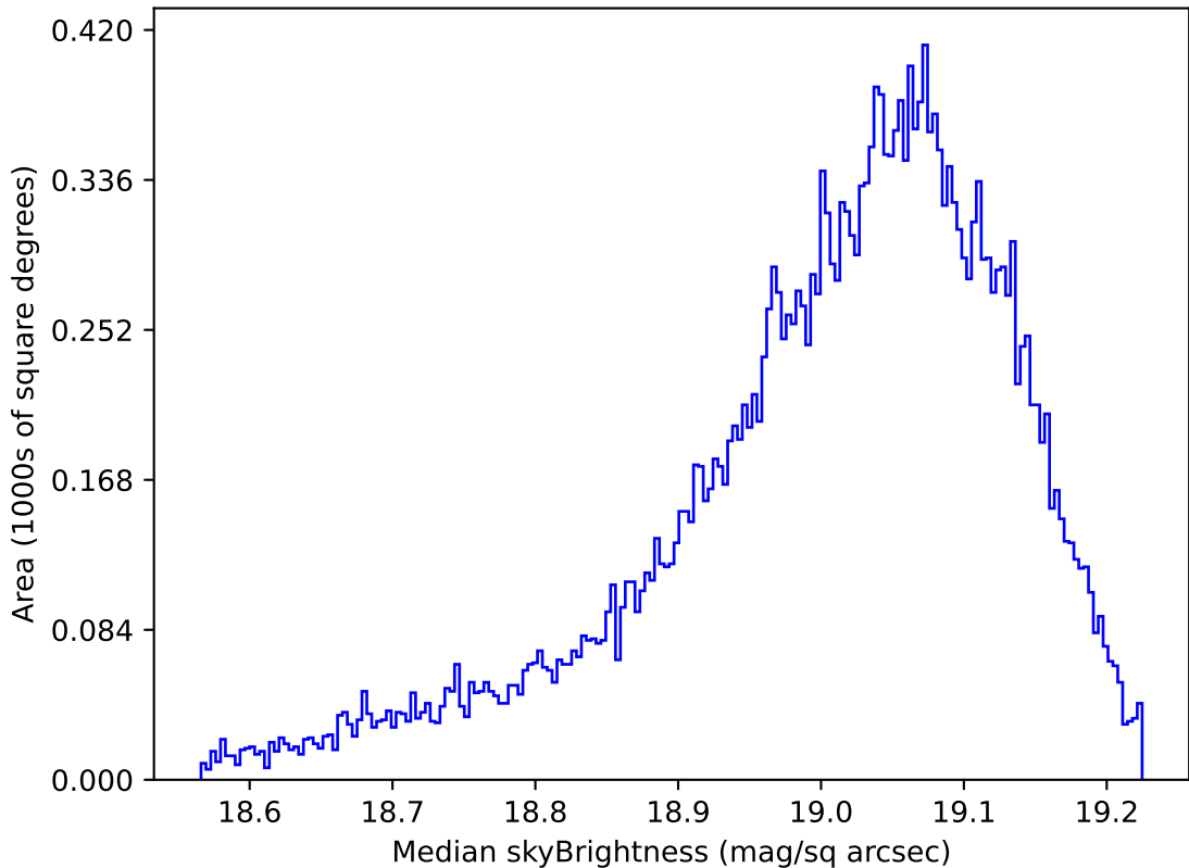
too_elab_r64_d3_gz_v3.4_10yrs All sky z band: Median skyBrightness
