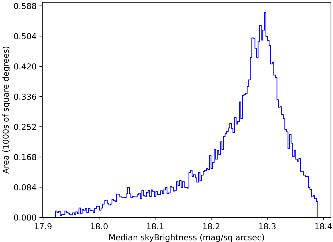
too_elab_r64_d3_gz_v3.4_10yrs All sky y band: Median skyBrightness
