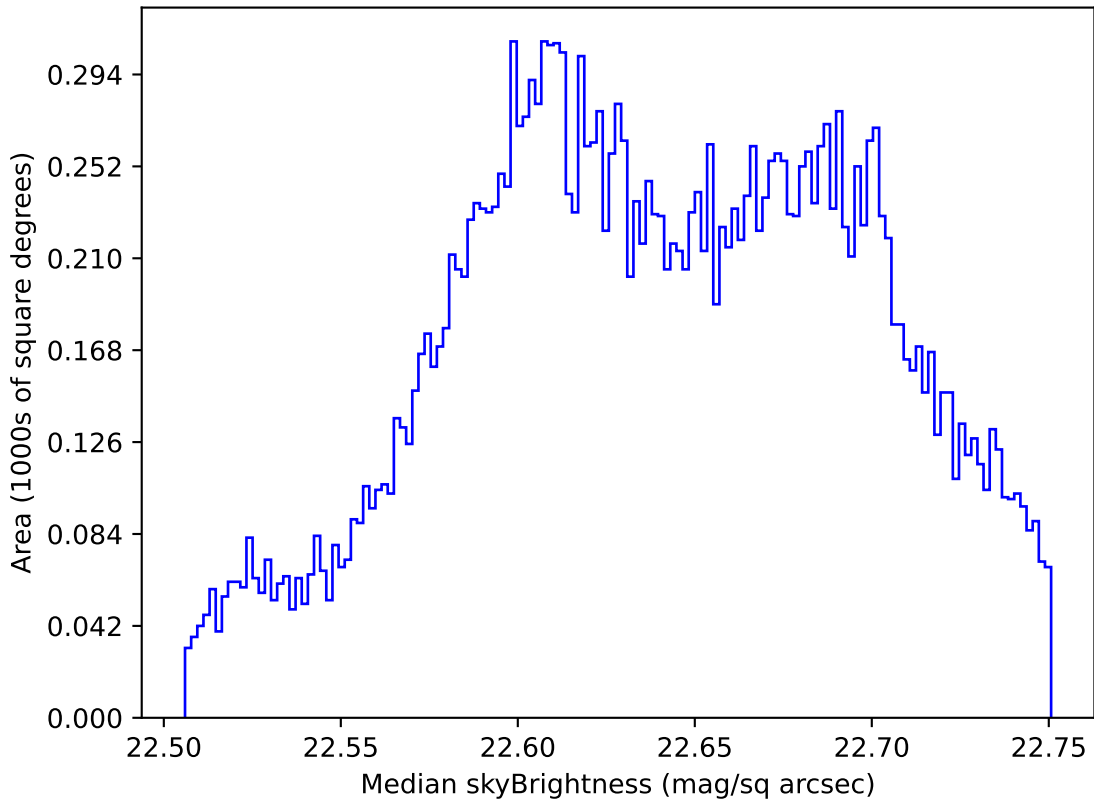
too_elab_r64_d3_gz_v3.4_10yrs All sky u band: Median skyBrightness
