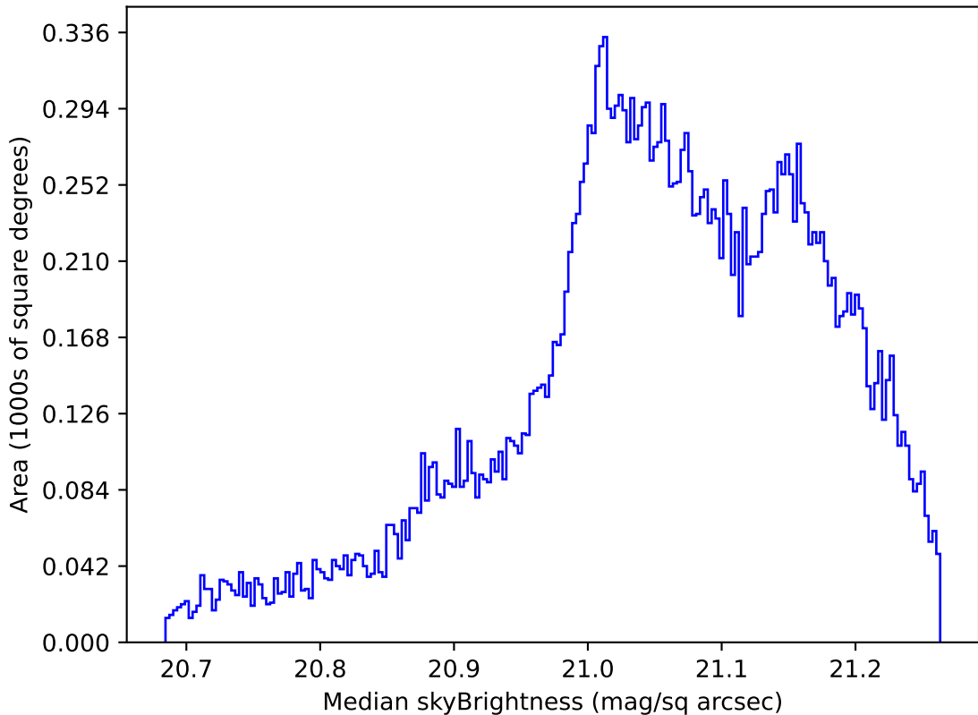
too_elab_r64_d3_gz_v3.4_10yrs All sky r band: Median skyBrightness
