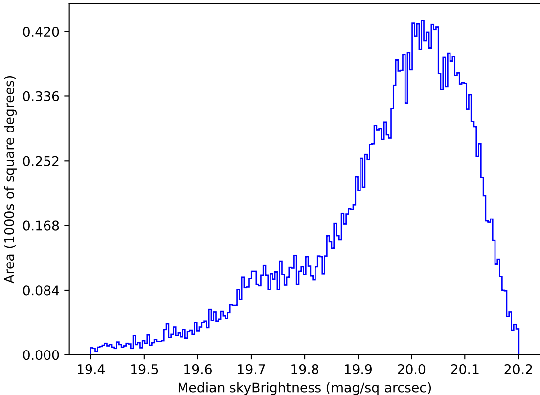
too_elab_r64_d3_gz_v3.4_10yrs All sky i band: Median skyBrightness
