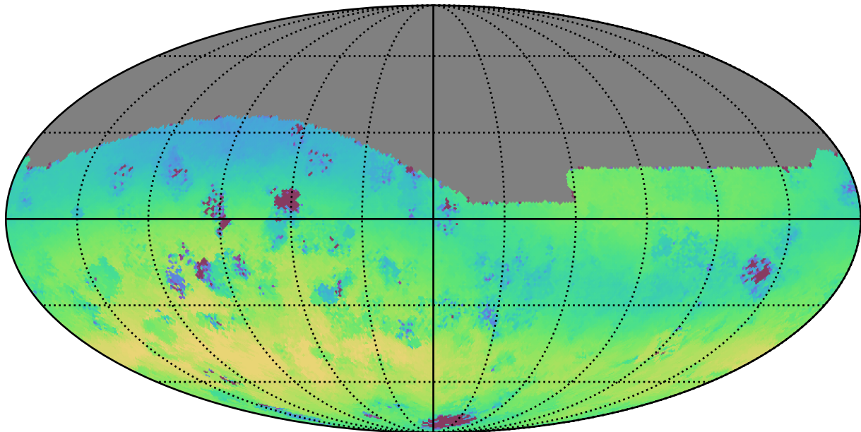
too_elab_r64_d3_gz_v3.4_10yrs All sky g band: Median skyBrightness
