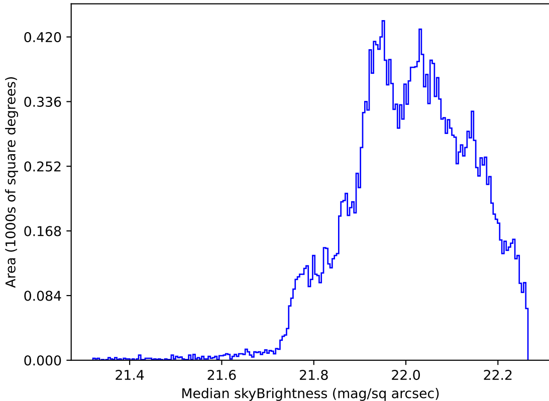
too_elab_r64_d3_gz_v3.4_10yrs All sky g band: Median skyBrightness
