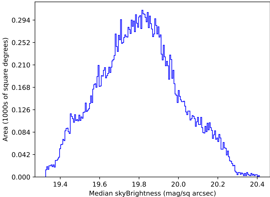
too_elab_r64_d3_gz_v3.4_10yrs All sky all bands: Median skyBrightness
