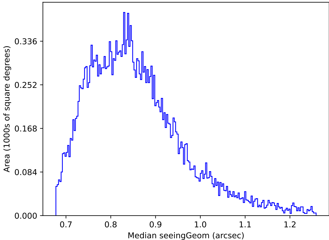
too_elab_r64_d3_gz_v3.4_10yrs Yr 1 z band: Median seeingGeom
