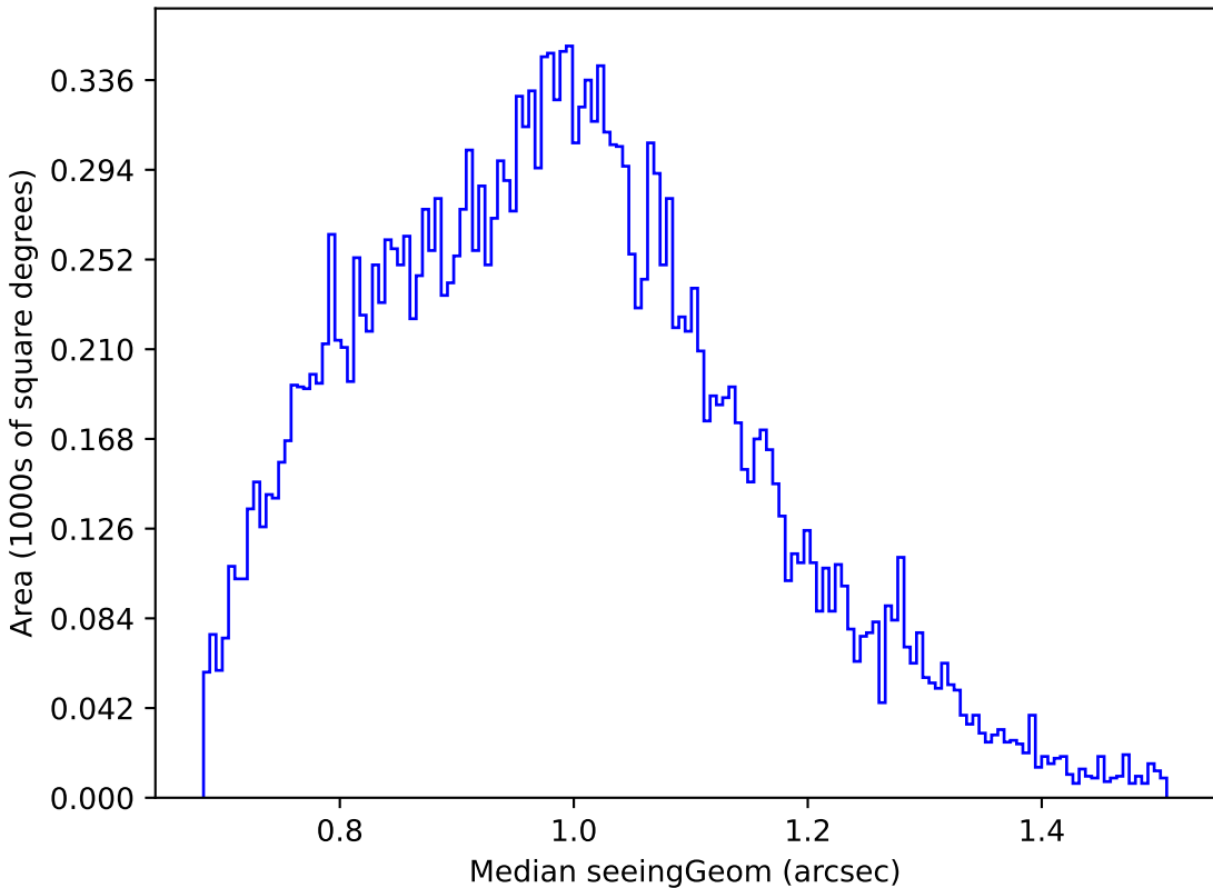
too_elab_r64_d3_gz_v3.4_10yrs Yr 1 u band: Median seeingGeom
