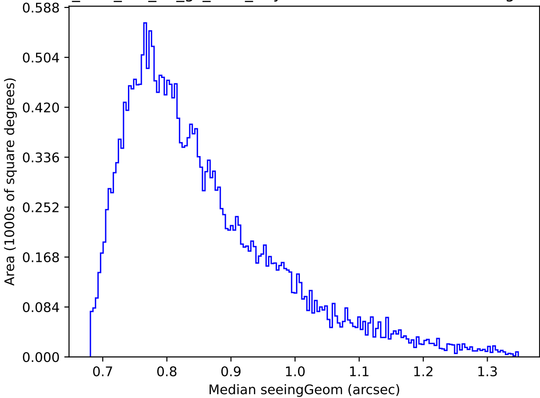
too_elab_r64_d3_gz_v3.4_10yrs Yr 1 r band: Median seeingGeom
