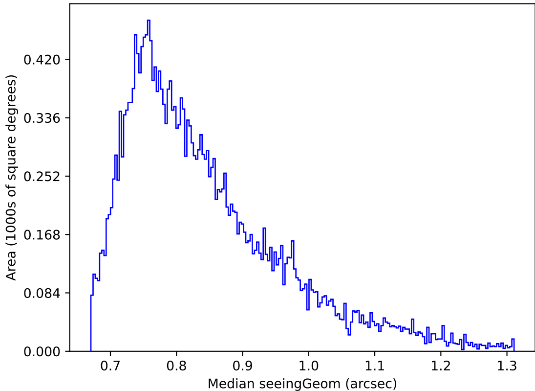
too_elab_r64_d3_gz_v3.4_10yrs Yr 1 i band: Median seeingGeom
