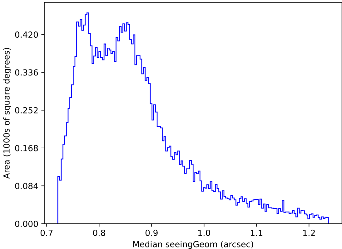
too_elab_r64_d3_gz_v3.4_10yrs Yr 1 all bands: Median seeingGeom
