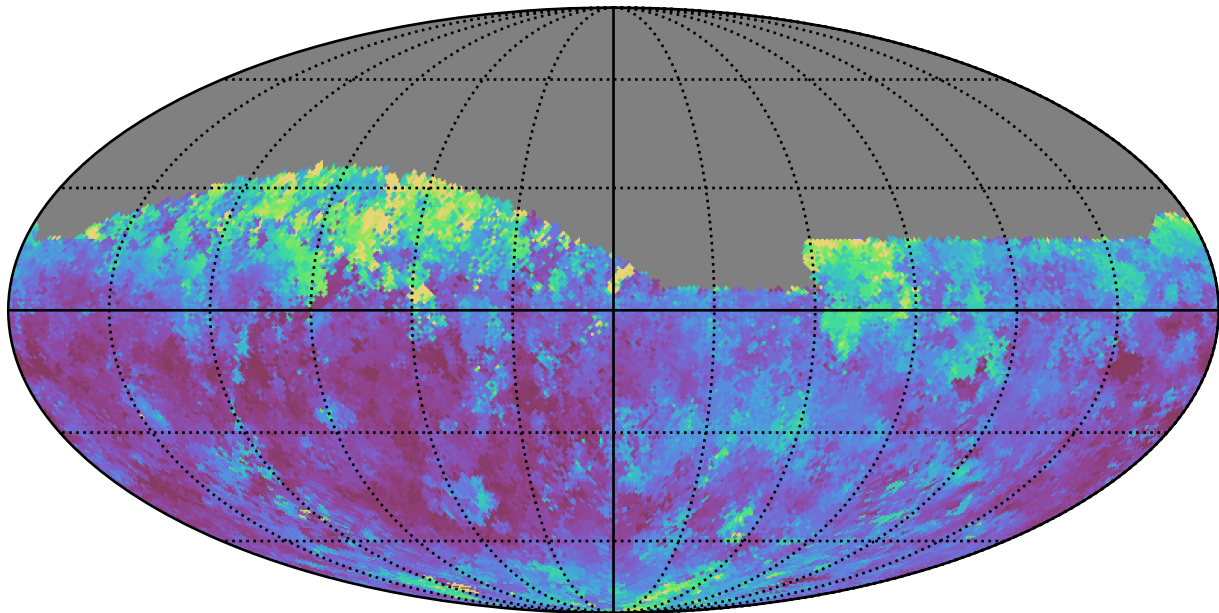
too_elab_r64_d3_gz_v3.4_10yrs Yr 1 z band: Median seeingEff
