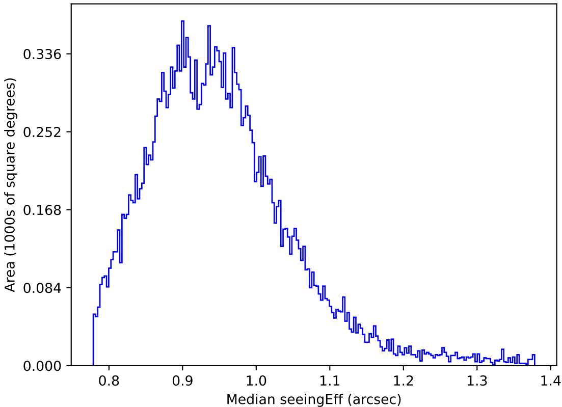
too_elab_r64_d3_gz_v3.4_10yrs Yr 1 y band: Median seeingEff
