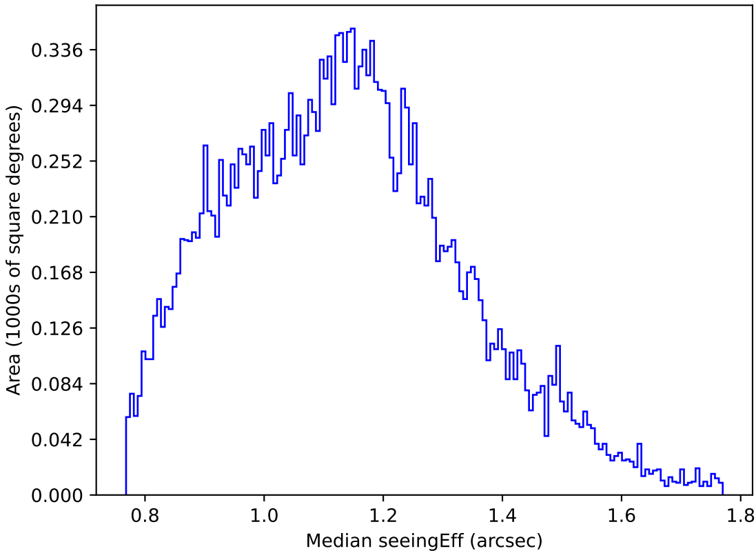
too_elab_r64_d3_gz_v3.4_10yrs Yr 1 u band: Median seeingEff
