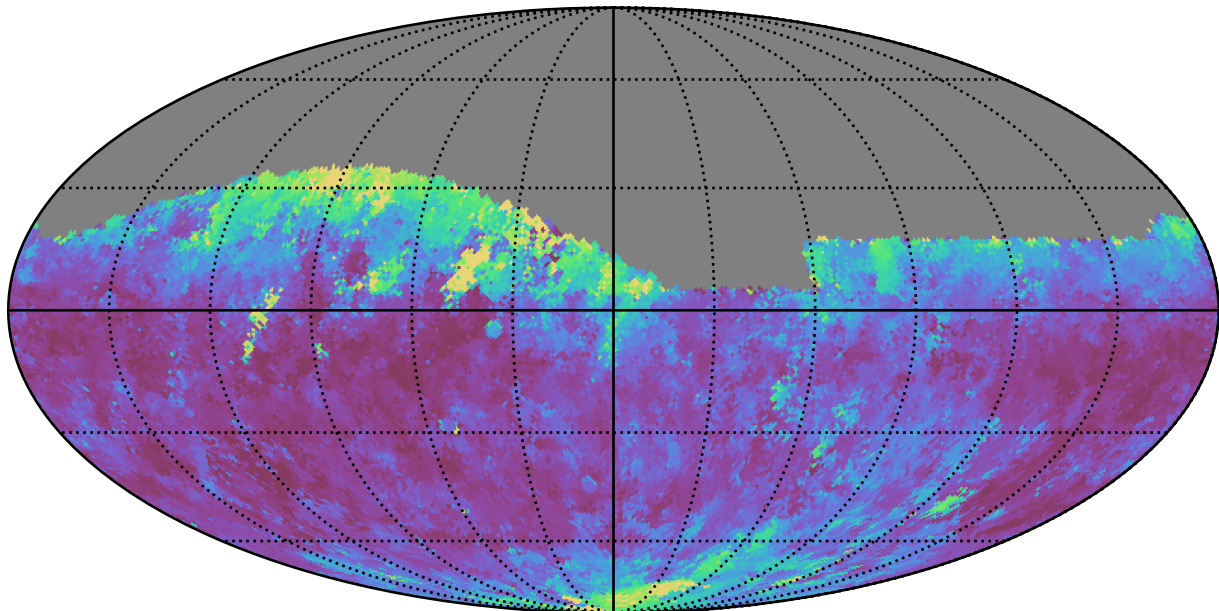
too_elab_r64_d3_gz_v3.4_10yrs Yr 1 r band: Median seeingEff
