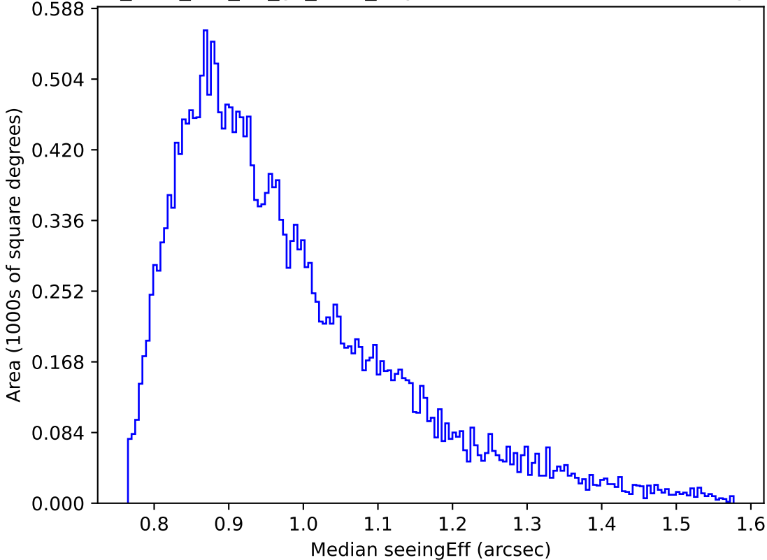
too_elab_r64_d3_gz_v3.4_10yrs Yr 1 r band: Median seeingEff
