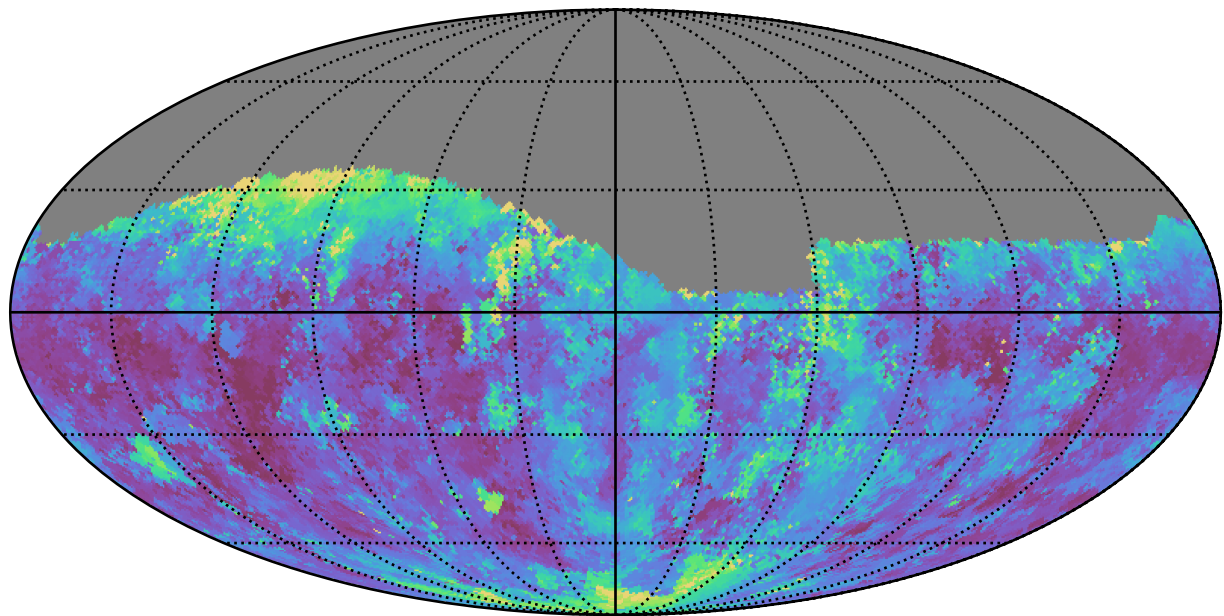
too_elab_r64_d3_gz_v3.4_10yrs Yr 1 g band: Median seeingEff
