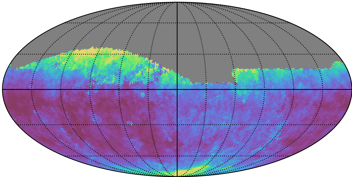
too_elab_r64_d3_gz_v3.4_10yrs Yr 1 all bands: Median seeingEff
