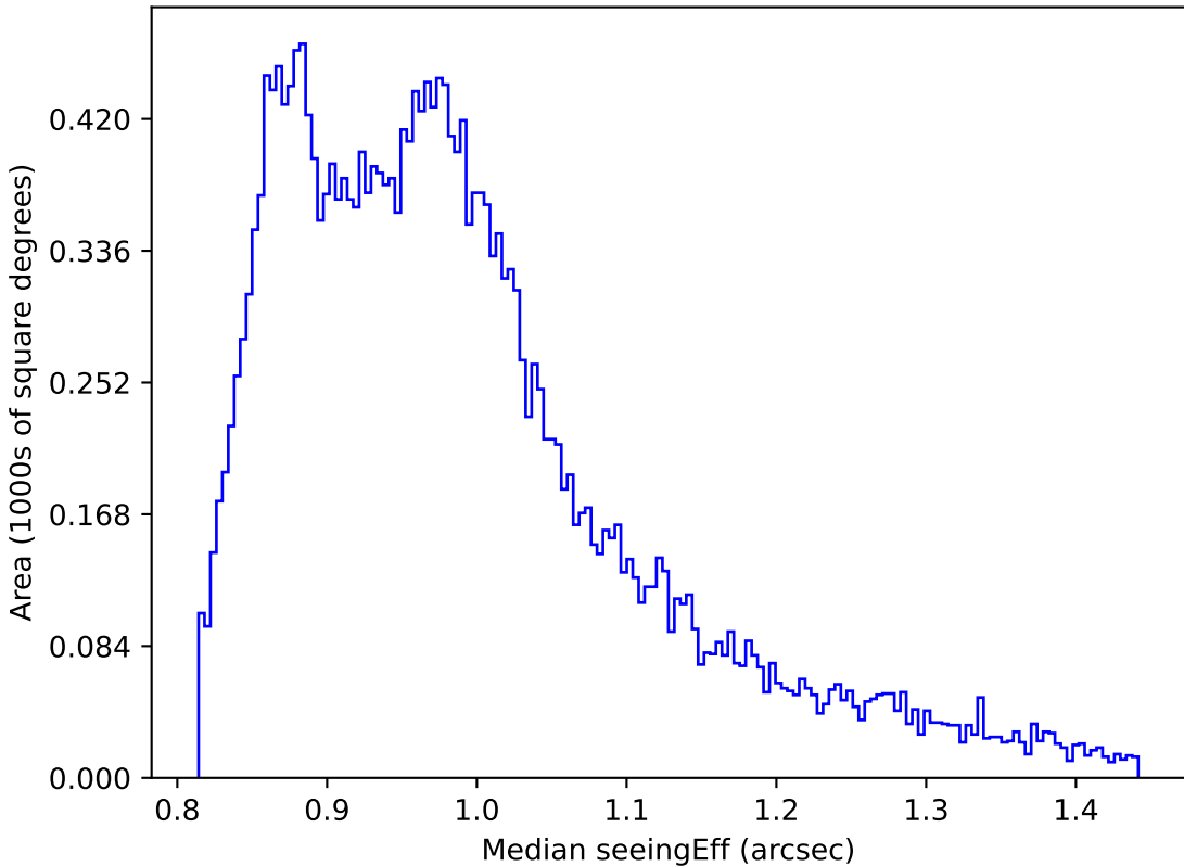
too_elab_r64_d3_gz_v3.4_10yrs Yr 1 all bands: Median seeingEff
