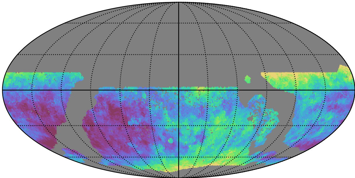
too_elab_r64_d3_gz_v3.4_10yrs WFD z band: Median seeingEff
