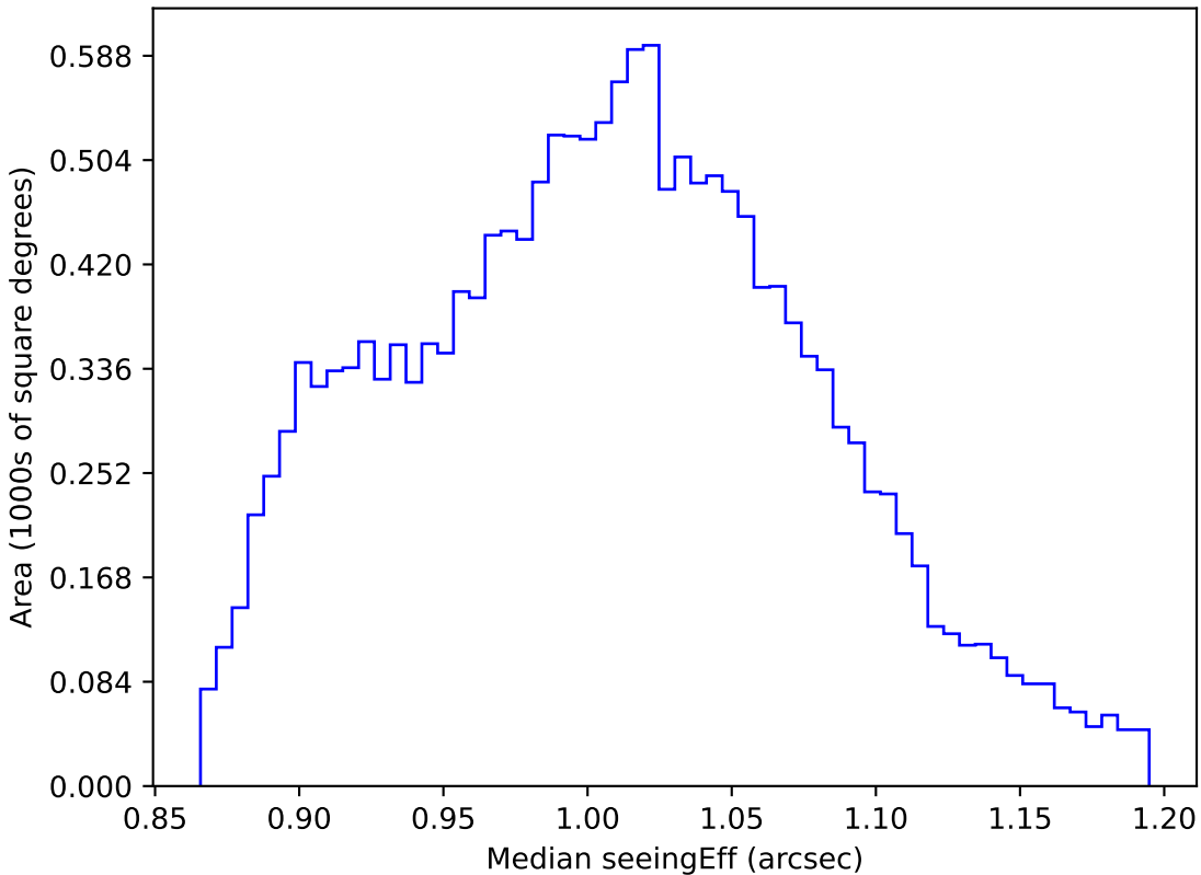
too_elab_r64_d3_gz_v3.4_10yrs WFD z band: Median seeingEff
