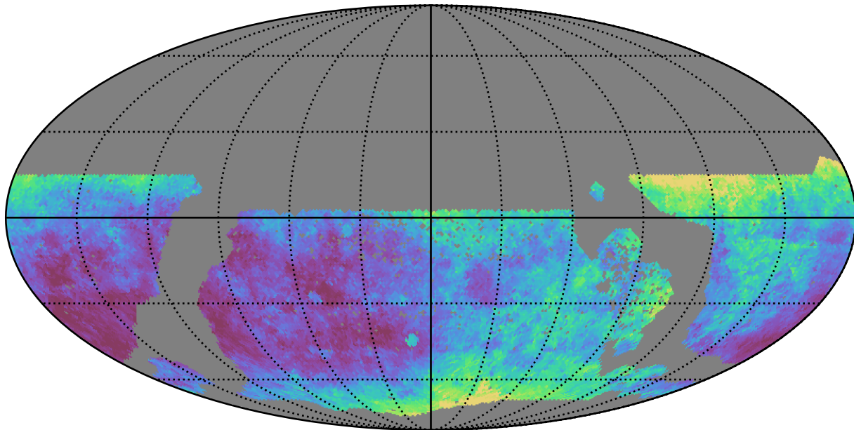
too_elab_r64_d3_gz_v3.4_10yrs WFD y band: Median seeingEff
