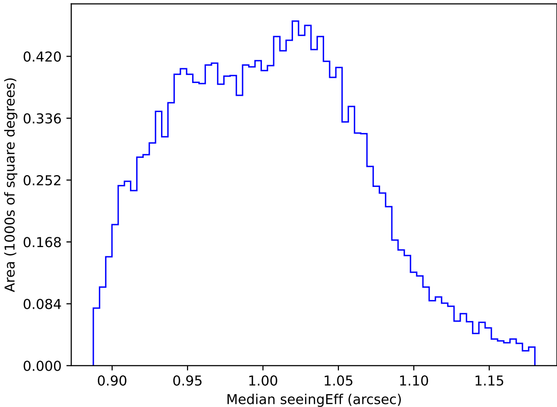
too_elab_r64_d3_gz_v3.4_10yrs WFD y band: Median seeingEff
