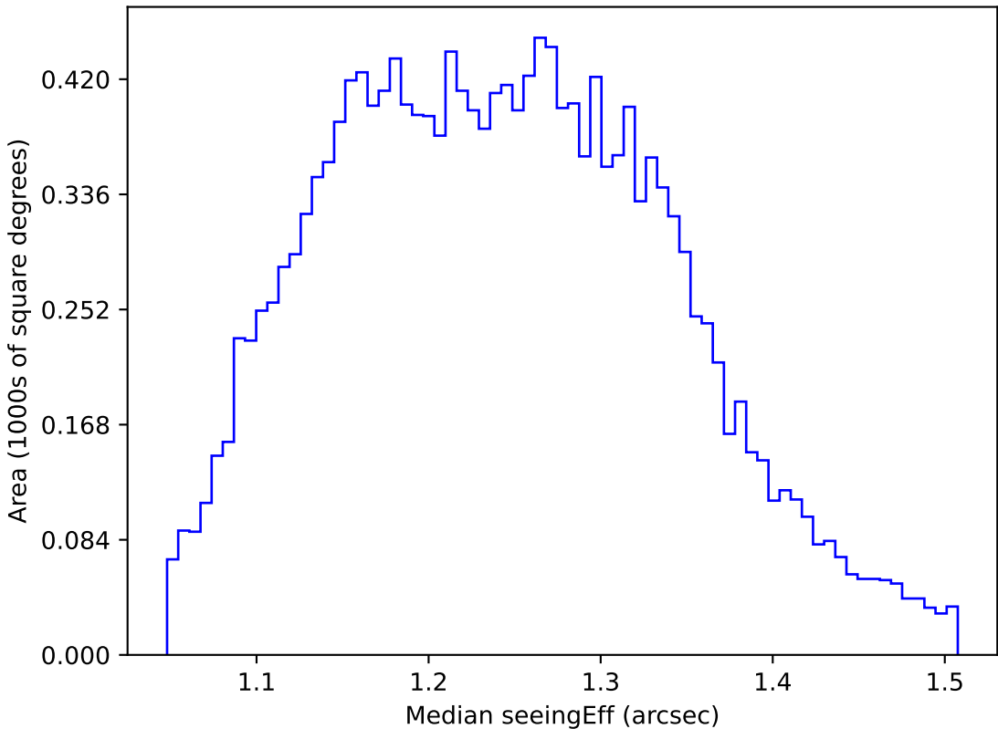
too_elab_r64_d3_gz_v3.4_10yrs WFD u band: Median seeingEff
