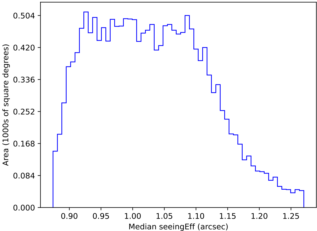
too_elab_r64_d3_gz_v3.4_10yrs WFD r band: Median seeingEff
