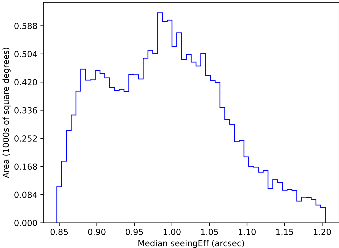
too_elab_r64_d3_gz_v3.4_10yrs WFD i band: Median seeingEff
