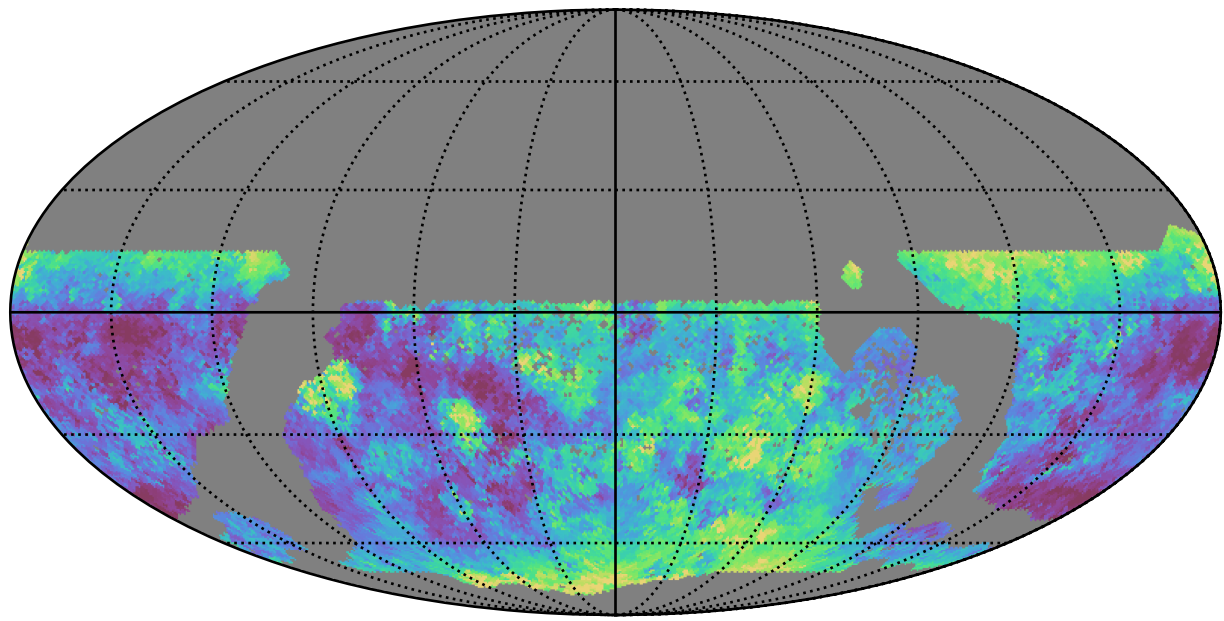
too_elab_r64_d3_gz_v3.4_10yrs WFD g band: Median seeingEff
