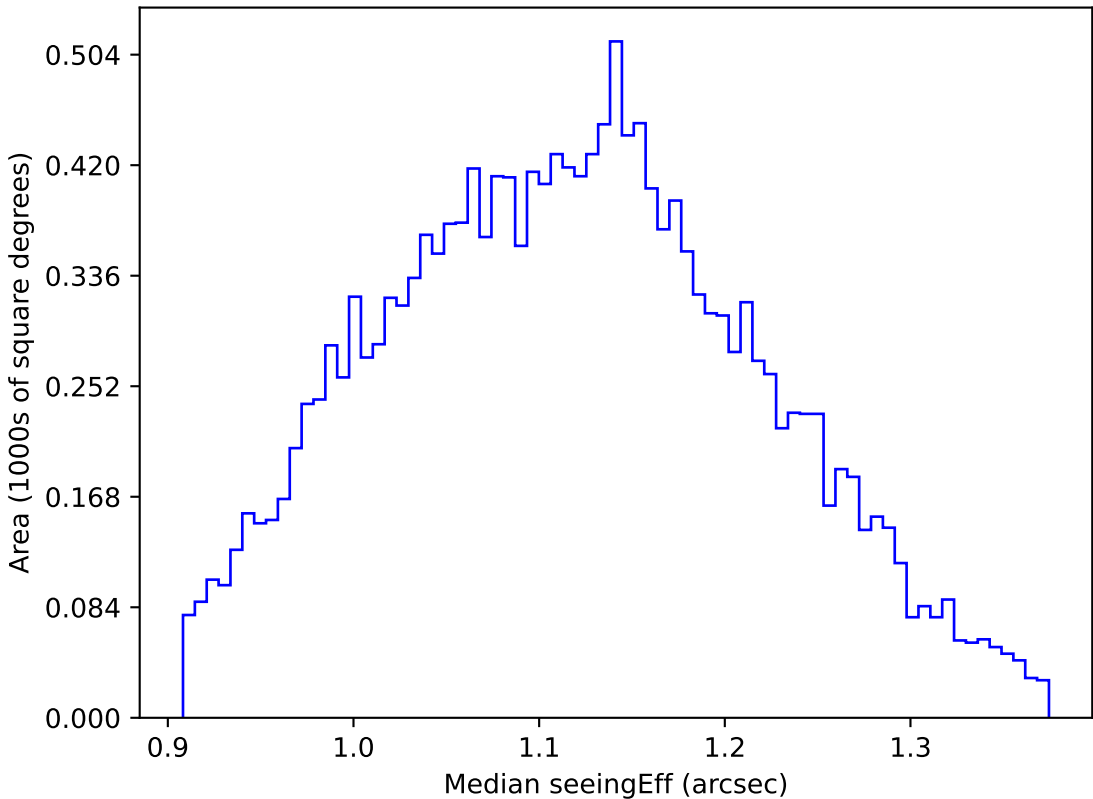
too_elab_r64_d3_gz_v3.4_10yrs WFD g band: Median seeingEff
