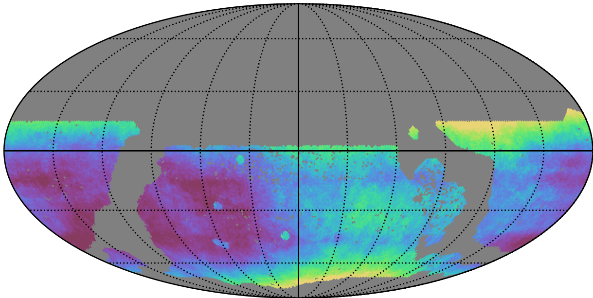
too_elab_r64_d3_gz_v3.4_10yrs WFD all bands: Median seeingEff
