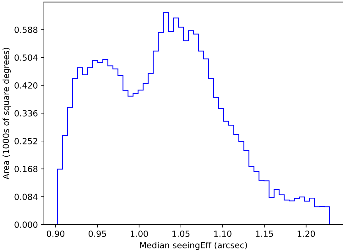
too_elab_r64_d3_gz_v3.4_10yrs WFD all bands: Median seeingEff
