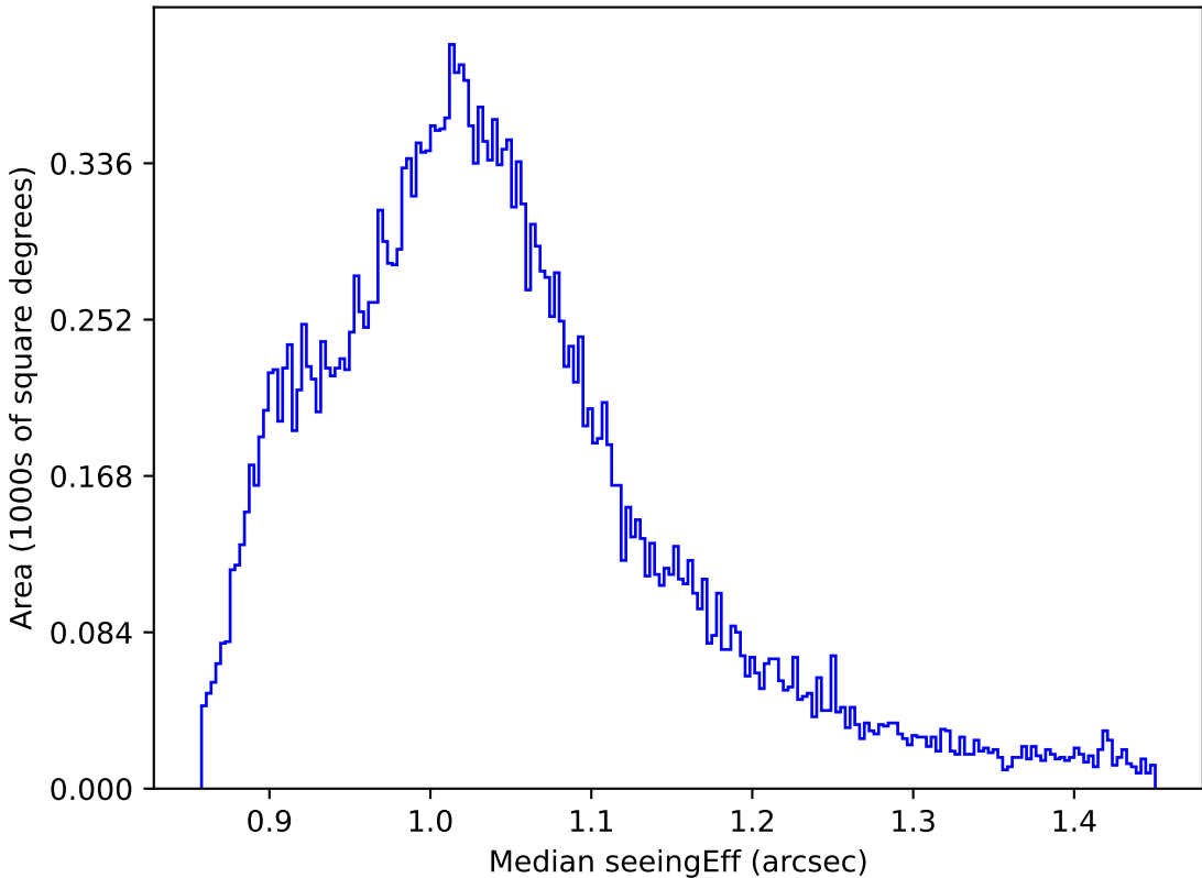
too_elab_r64_d3_gz_v3.4_10yrs All sky z band: Median seeingEff
