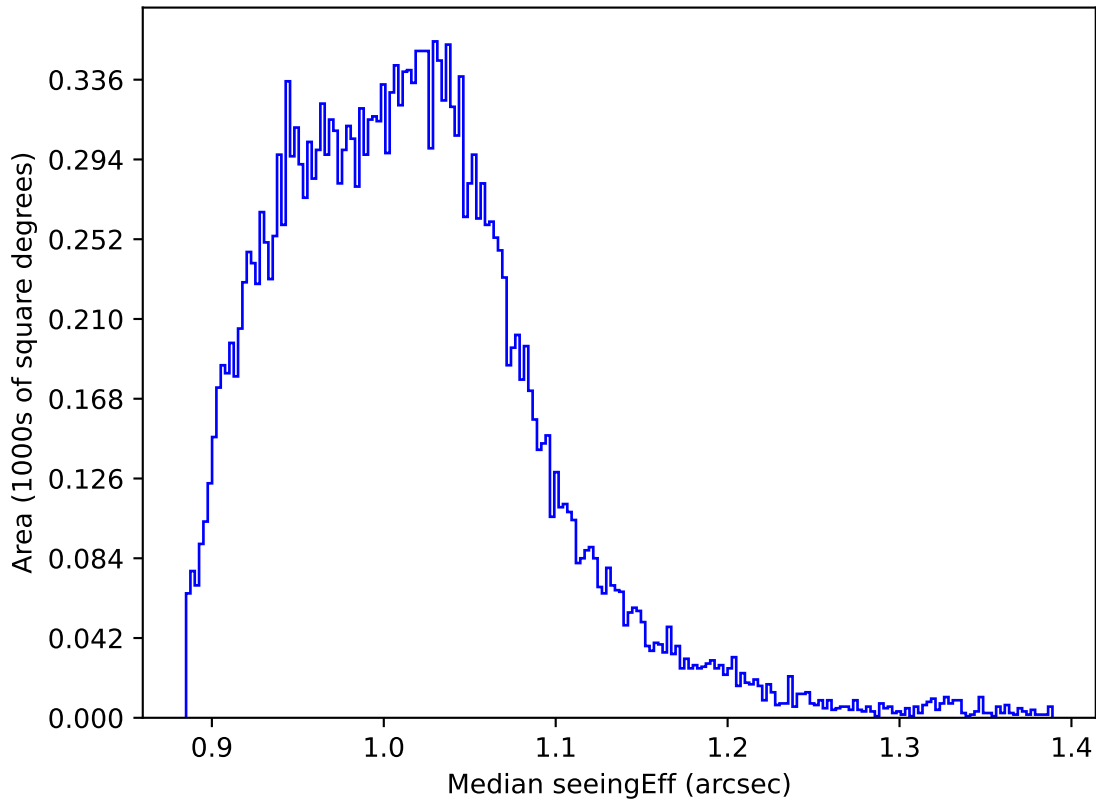
too_elab_r64_d3_gz_v3.4_10yrs All sky y band: Median seeingEff
