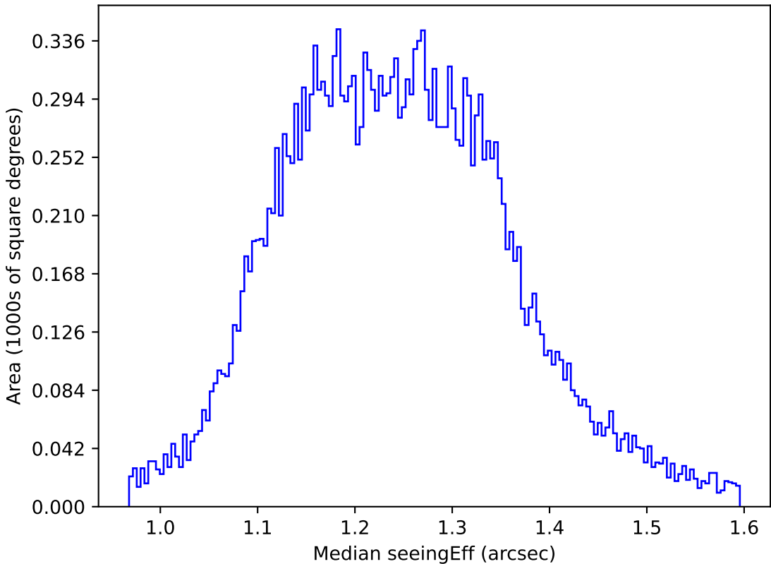
too_elab_r64_d3_gz_v3.4_10yrs All sky u band: Median seeingEff
