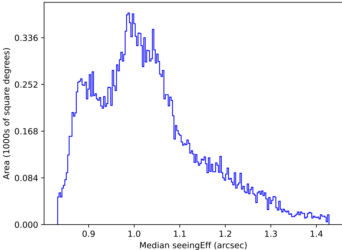
too_elab_r64_d3_gz_v3.4_10yrs All sky i band: Median seeingEff
