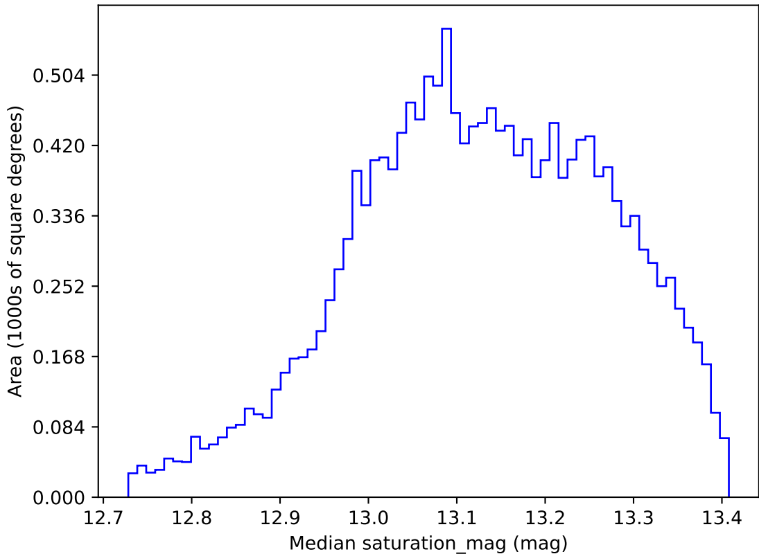
too_elab_r64_d3_gz_v3.4_10yrs WFD y band: Median saturation_mag
