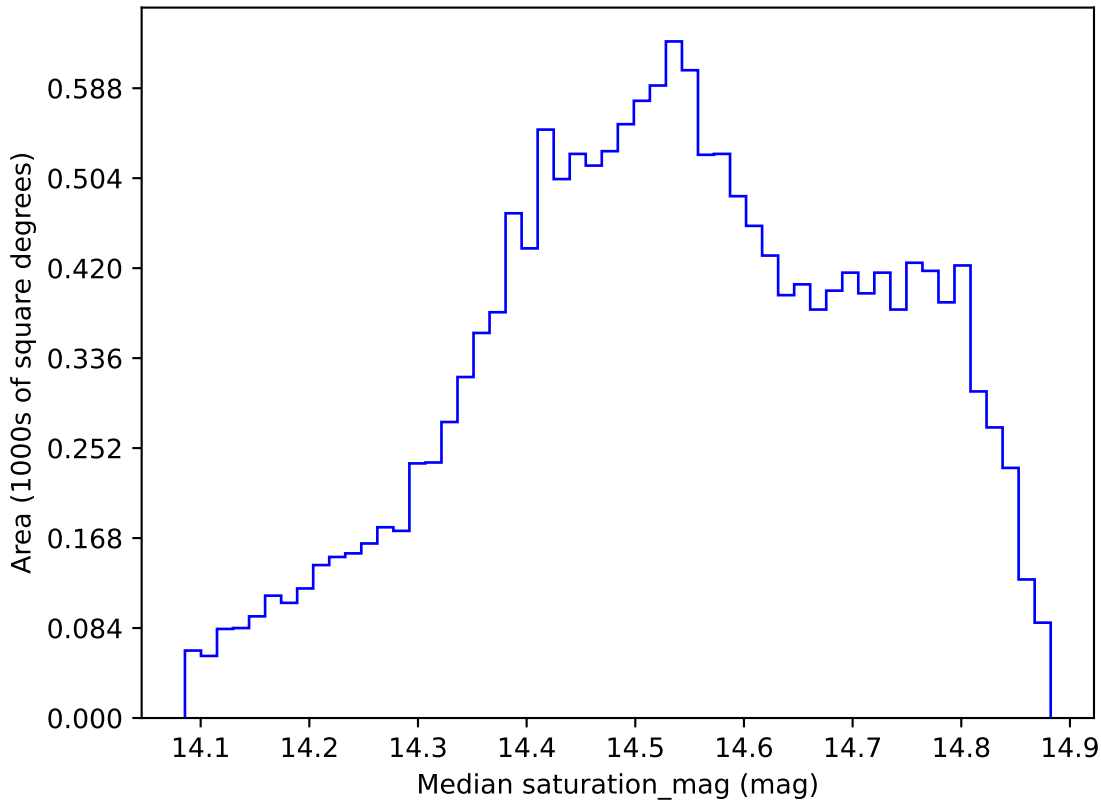
too_elab_r64_d3_gz_v3.4_10yrs WFD i band: Median saturation_mag
