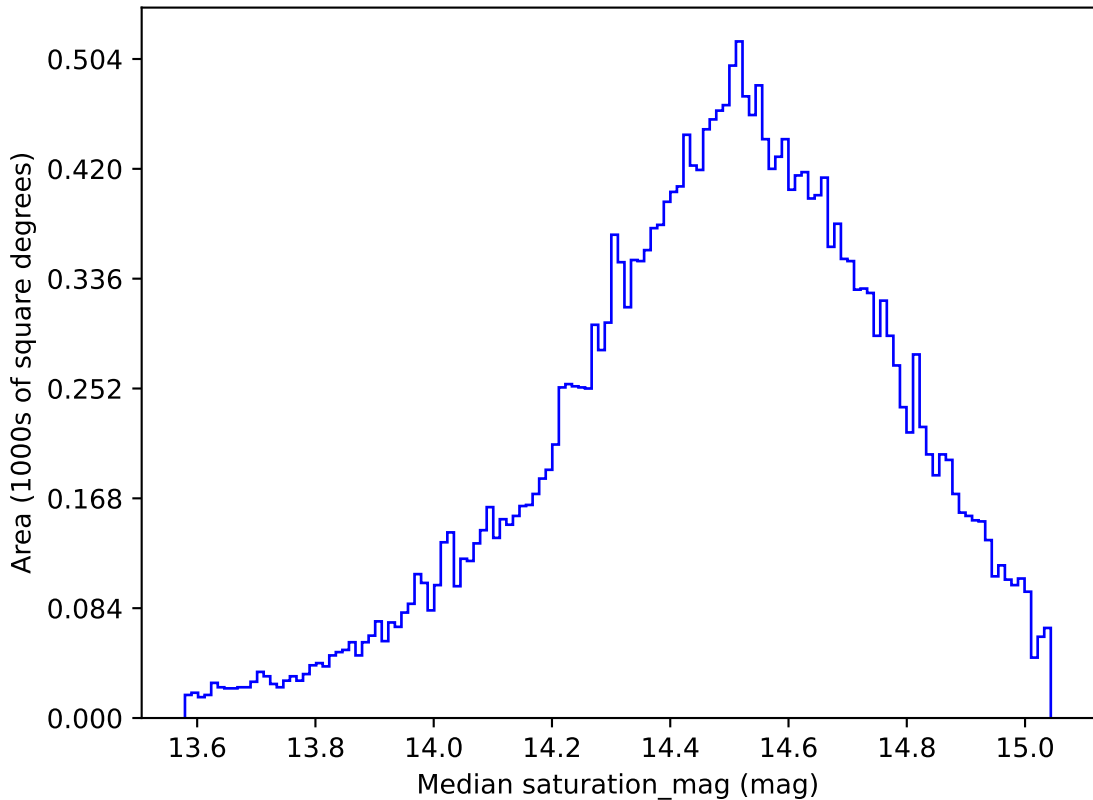
too_elab_r64_d3_gz_v3.4_10yrs All sky g band: Median saturation_mag
