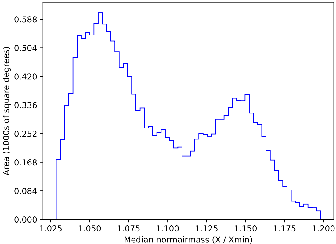
too_elab_r64_d3_gz_v3.4_10yrs WFD y band: Median normairmass
