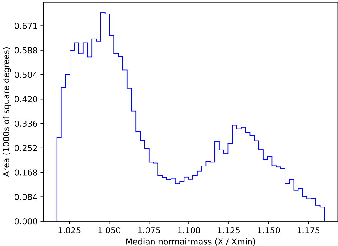
too_elab_r64_d3_gz_v3.4_10yrs WFD r band: Median normairmass
