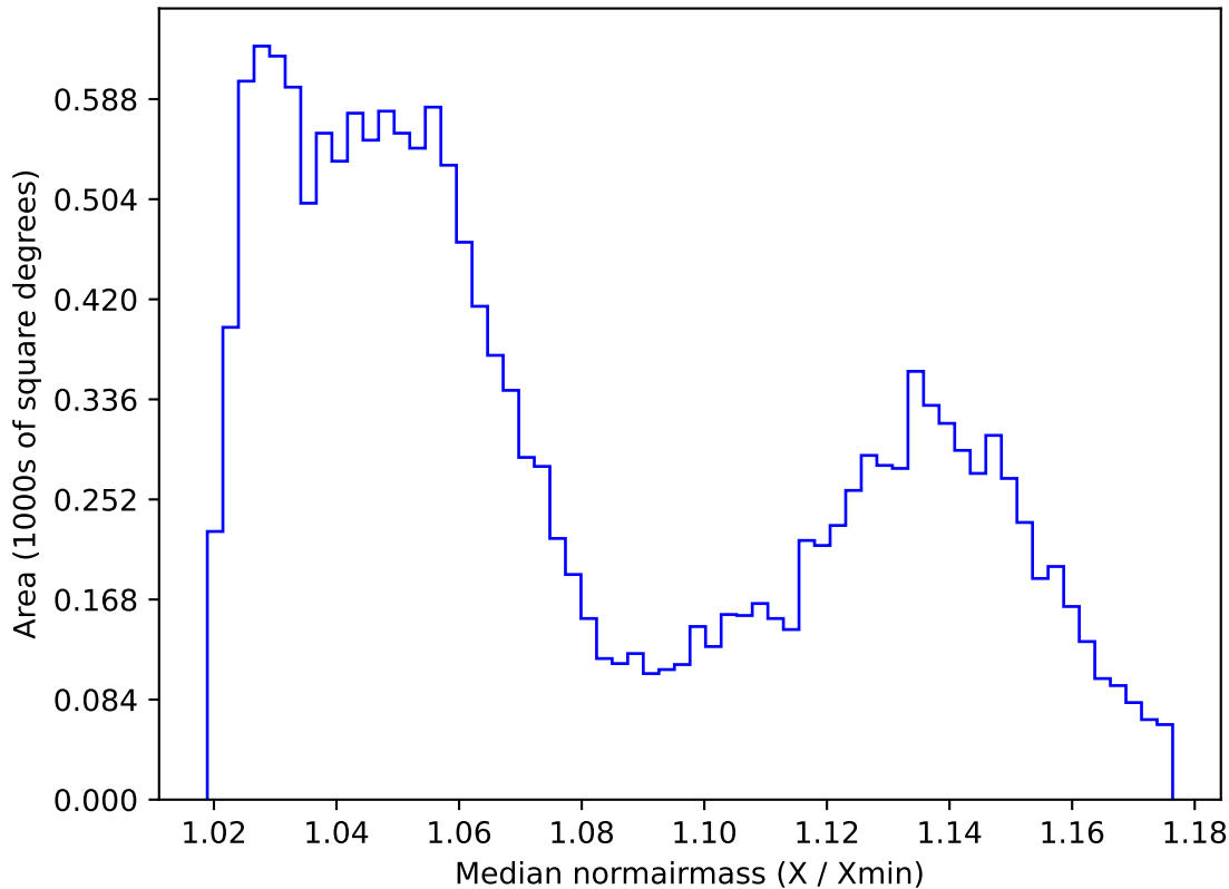
too_elab_r64_d3_gz_v3.4_10yrs WFD i band: Median normairmass
