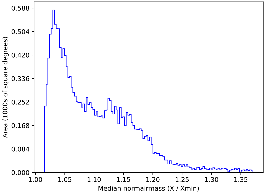
too_elab_r64_d3_gz_v3.4_10yrs WFD g band: Median normairmass
