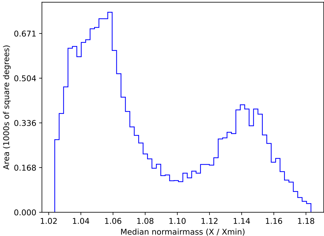
too_elab_r64_d3_gz_v3.4_10yrs WFD all bands: Median normairmass
